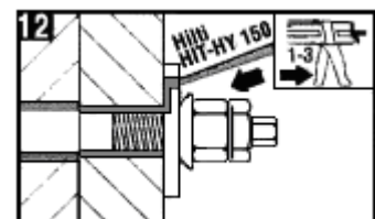
12 Inject the HIT resin through the hole in the top of the injection washer.
